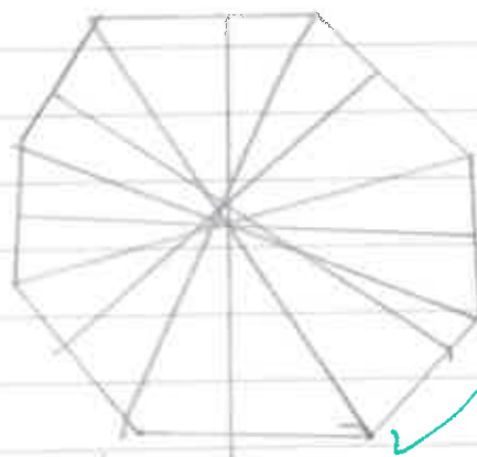
Lines of symmetry 8 octagon
