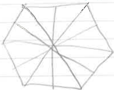
Lines of symmetry 6 hexagon
