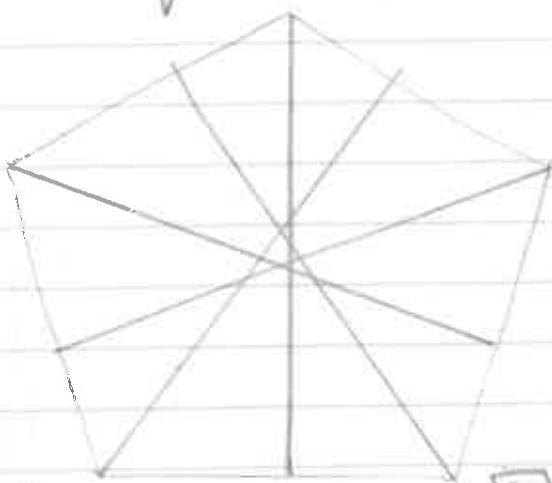
Lines of symmetry 5 pentagon
