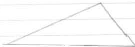
Lines of symmetry 1 isosceles
